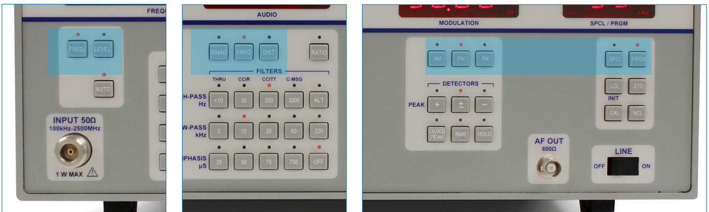
Figure-4: Function Keys of 8201A Modulation Analyzer
