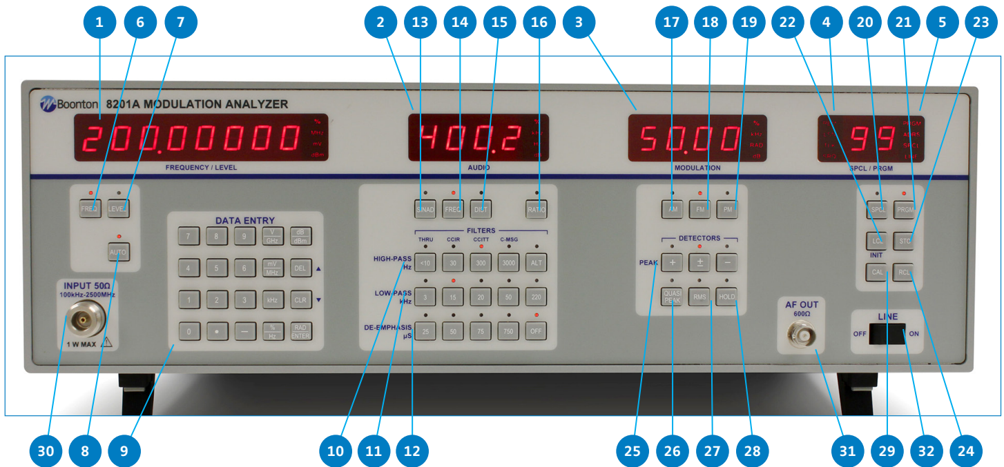
Figure-2: Front View of 8201A Modulation Analyzer
