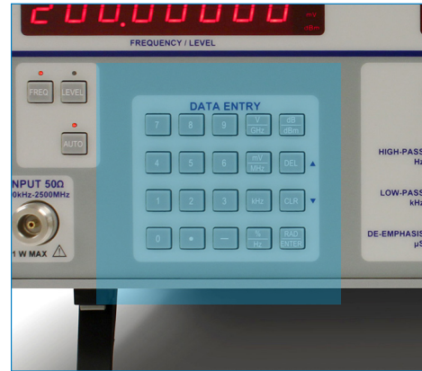
Figure-5: Data Keypad of 8201A Modulation Analyzer
