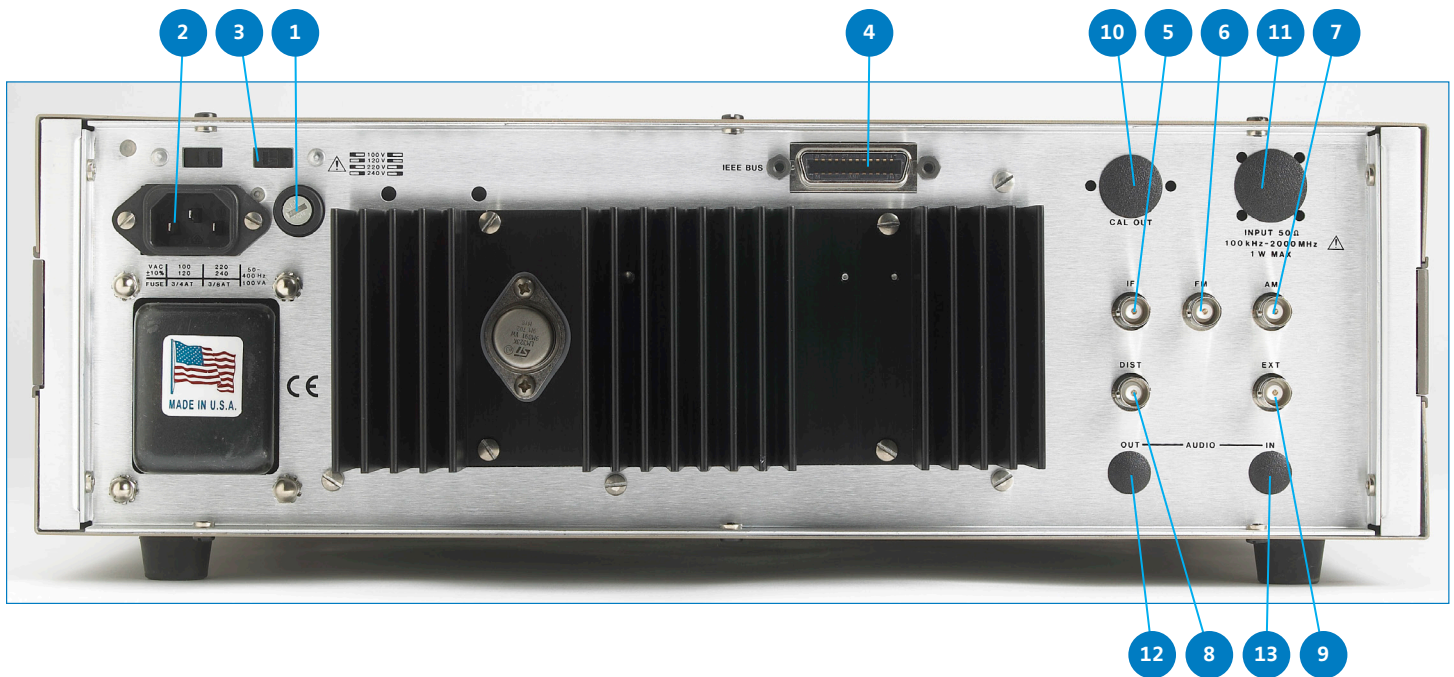
Figure-3: Rear View of 8201A Modulation Analyzer
