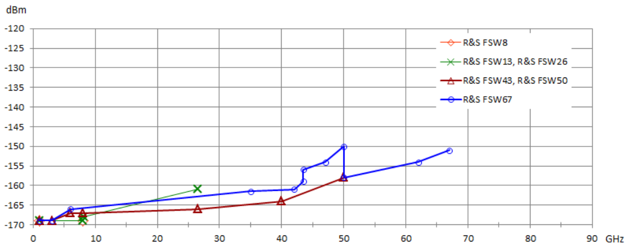
Typical displayed average noise level of the R&S®FSW models for f > 1 GHz with R&S®FSW-B24 9 RF preamplifier option, preamplifier gain = 30 dB.
