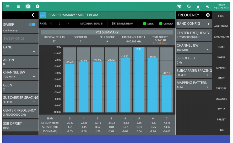
Measurement summary screen displays essential results to validate base station performance
