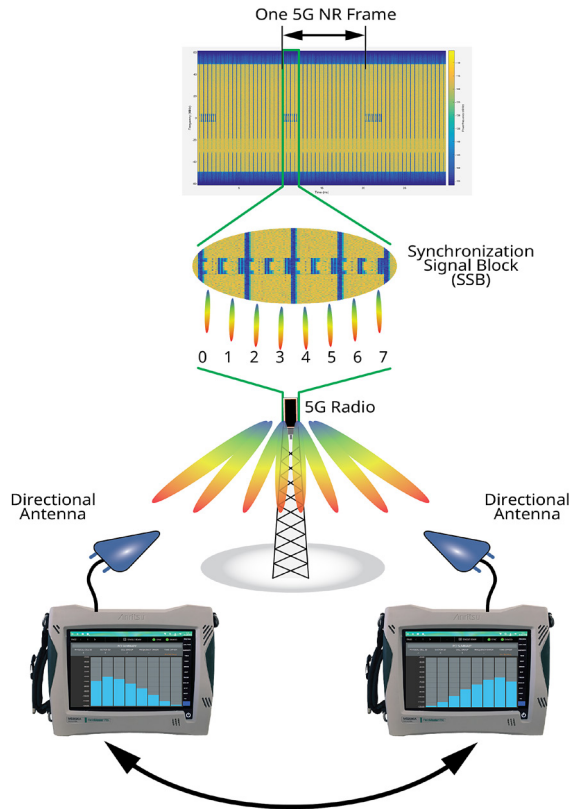
Field Master Pro MS2090A displays RSRP vs beam index based on OTA analysis of the 5G NR SSB
