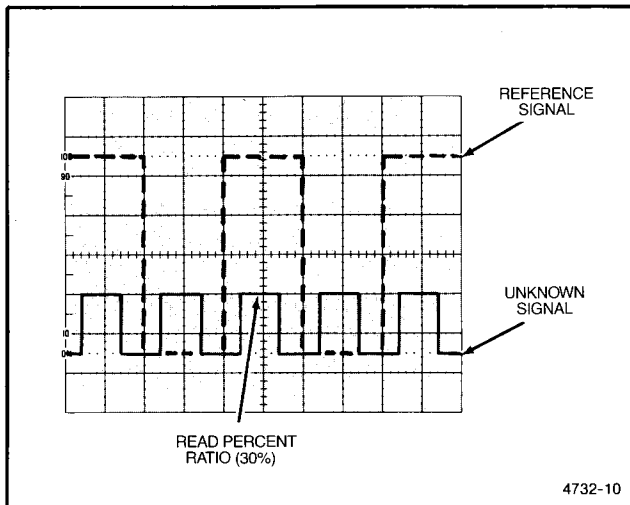
Figure 3-4. Determining voltage ratio.
