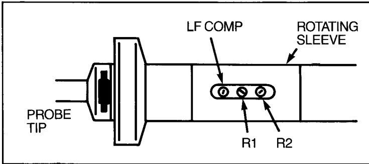
Figure 4-2. Locating the low-frequency compensation adjustment.
