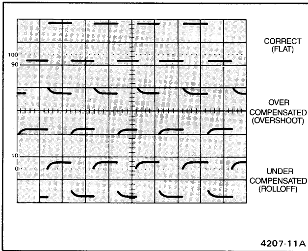
Figure 4-1. Probe compensation.
